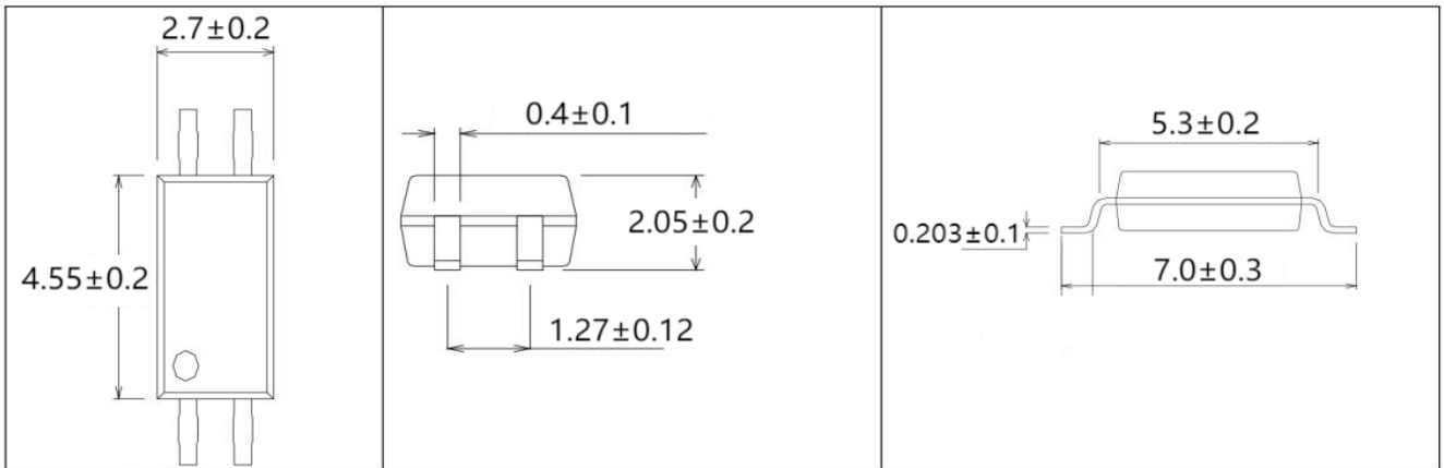
4-pin SSOP
