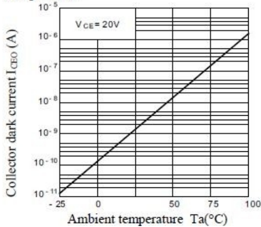
Fig.7 Collector Dark Current vs. Ambient Temperature
