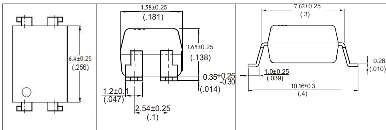
4-pin SMD
