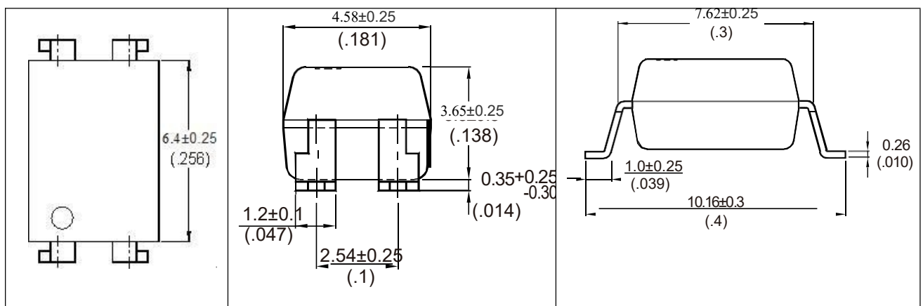
4-pin SMD
