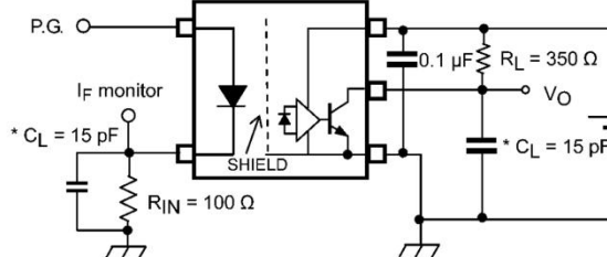
Fig.5: Switching Time Test Circuit and Waveform
